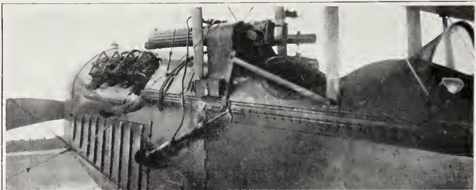
SHOOTING THROUGH PROPELLER.
