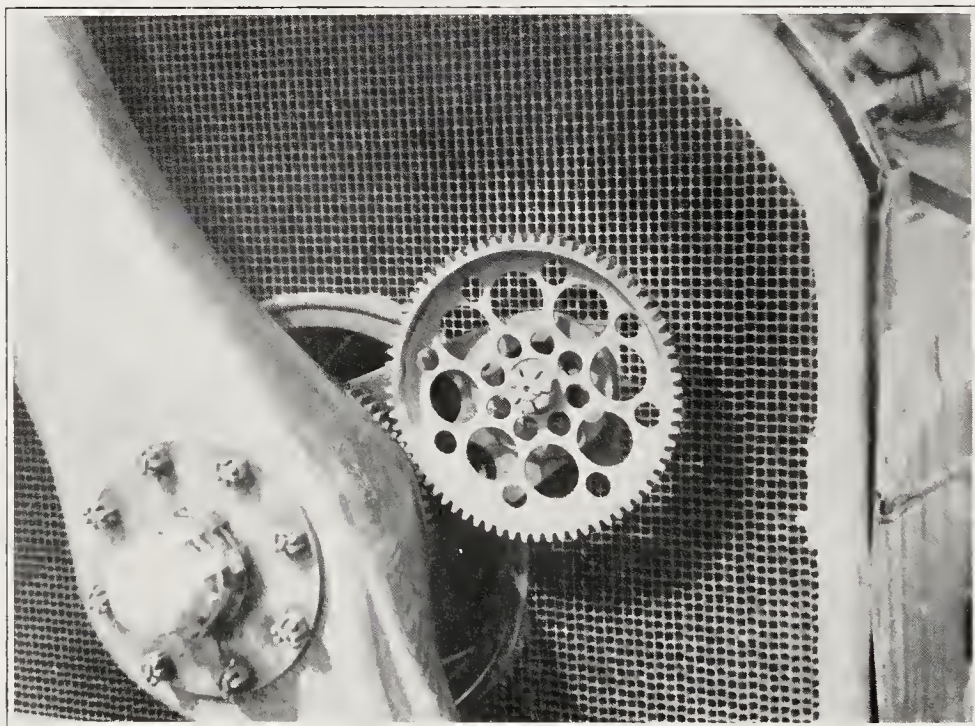
SYNCHRONIZING GEAR.
