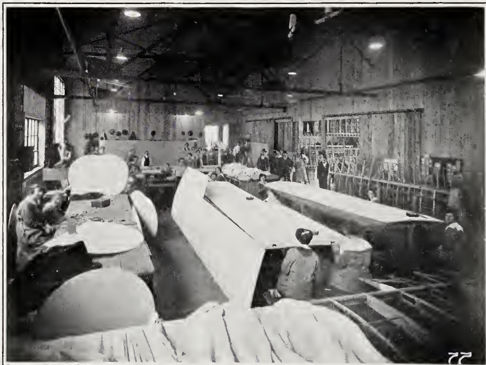
SAILMAKING ON WINGS.
