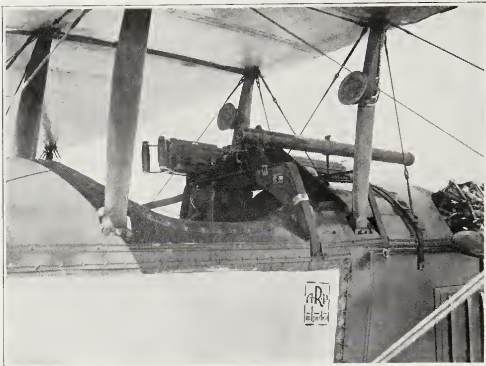
SYNCHRONIZED VICKERS' GUN.
