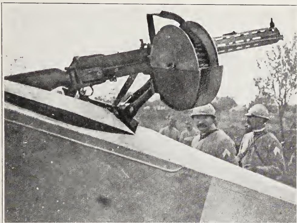
GERMAN PARABELLUM MOUNTING.
