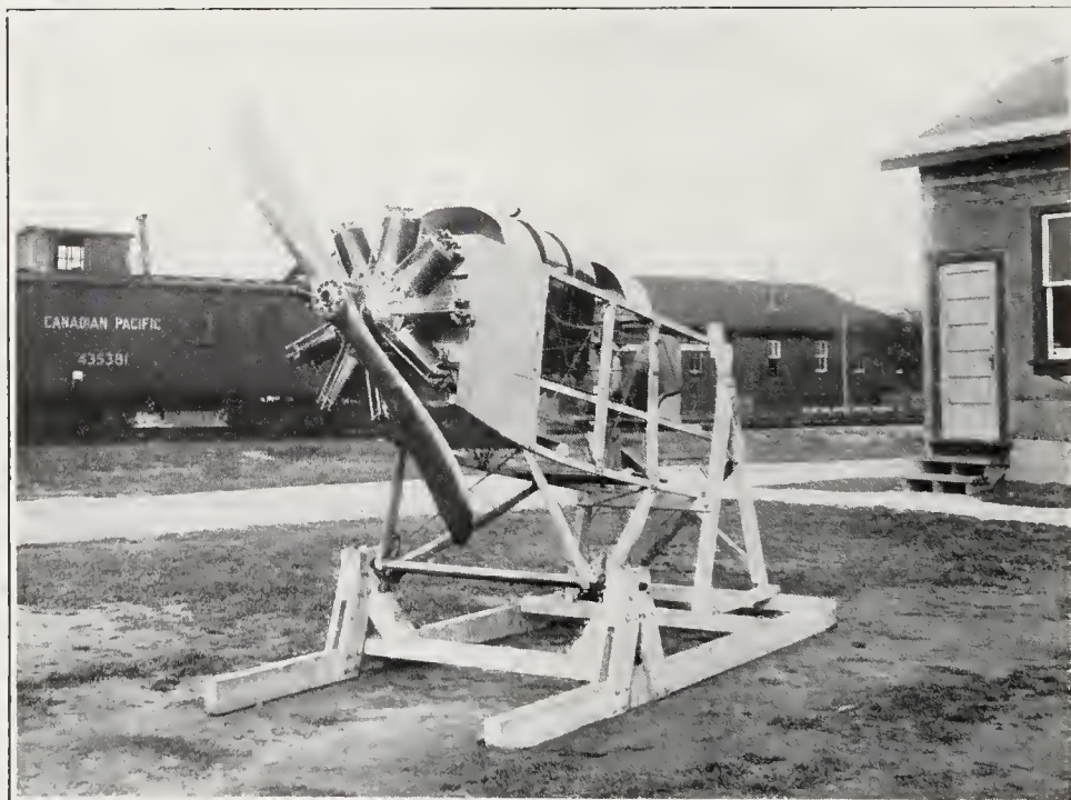
CLERGET ENGINE ON ROCKING NACELLE.
