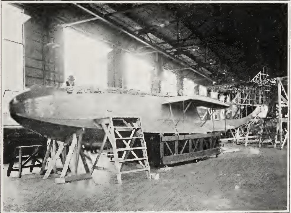
FLYING BOAT HULL UNDER CONSTRUCTION.
