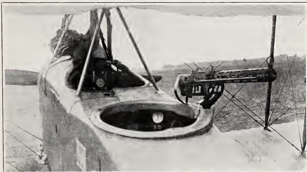
OBSERVERS' GUN MOUNTING
